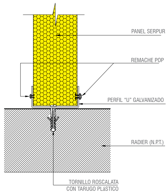
Muro Interior
